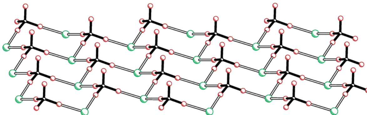
Figure 4. The two-dimensional honeycombed donor/acceptor layer in the structure of [\text{Bu}_4\text{N}^+\text{Br}^-\cdot\text{CBr}_4] as the result of fragmentation of the three-dimensional diamondoid network shown in Figure 2. Note: the noncentrosymmetric structure is polarized across the mean plane.
