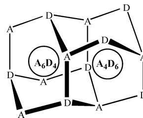
Figure 2. The diamondoid donor/acceptor network in the structures of [\text{Et}_4\text{N}^+\text{halide}^-\text{CBr}_4] complexes. In all figures, the halide anions are shown as green circles, and the donor/acceptor bonds are shown as empty lines. The \text{Et}_4\text{N}^+ counterions are omitted for clarity.
