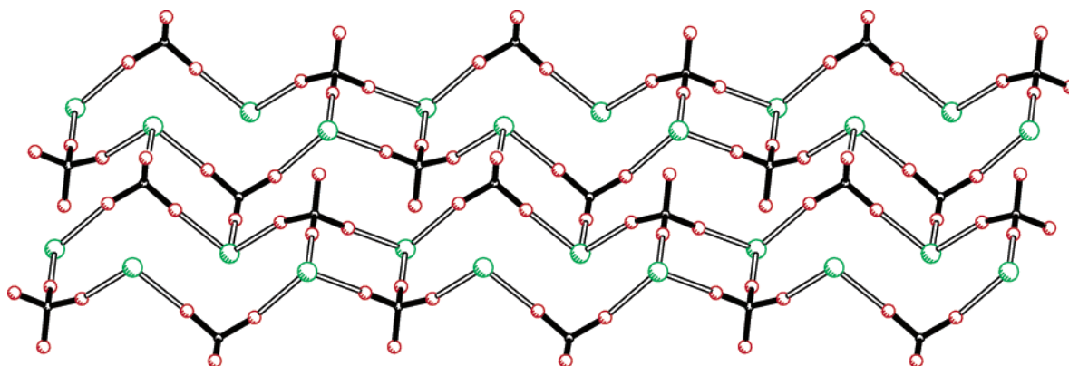
Figure 6. The two-dimensional centrosymmetric donor/acceptor layer in the structure of [\text{DBU}-\text{H}^+\text{Br}^-, \text{CBr}_4] distorted by competition with H-bonding in the crystal, see text.
