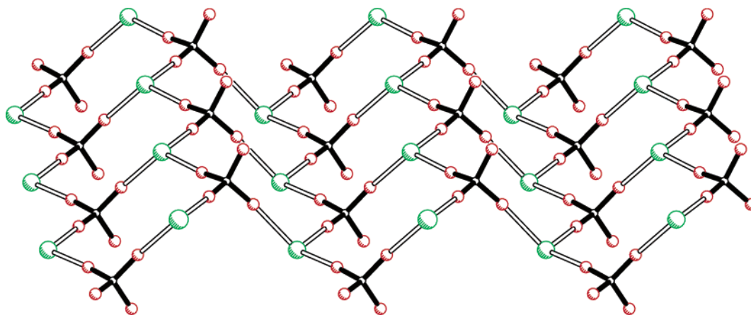
Figure 5. The two-dimensional folded donor/acceptor layer in the structure of [\text{Pr}_4\text{N}^+\text{Br}^-, \text{CBr}_4] as the product of the rearrangement of the two-dimensional “diamondoid” layer in Figure 4. Note: the noncentrosymmetric structure is polarized along the mean plane.
