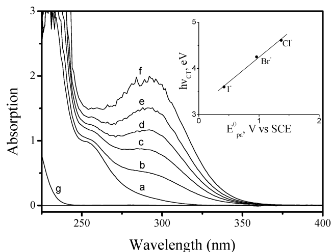
Figure 1. Spectral changes attendant upon the addition of tetrapropylammonium bromide to a 7.5 mM solution of carbon tetrabromide in dichloromethane at 22 °C. Concentration of \text{Pr}_4\text{N}^+\text{Br}^- [mM]: (a) 0; (b) 18; (c) 38; (d) 56; (e) 75; (f) 94. For comparison: (g) is the spectrum of 50 mM \text{Pr}_4\text{N}^+\text{Br}^- alone. Inset: Mulliken correlation between the energy of the charge-transfer band and the oxidation potential of the donor in the complexes of \text{CBr}_4 acceptor with halides (as indicated).
